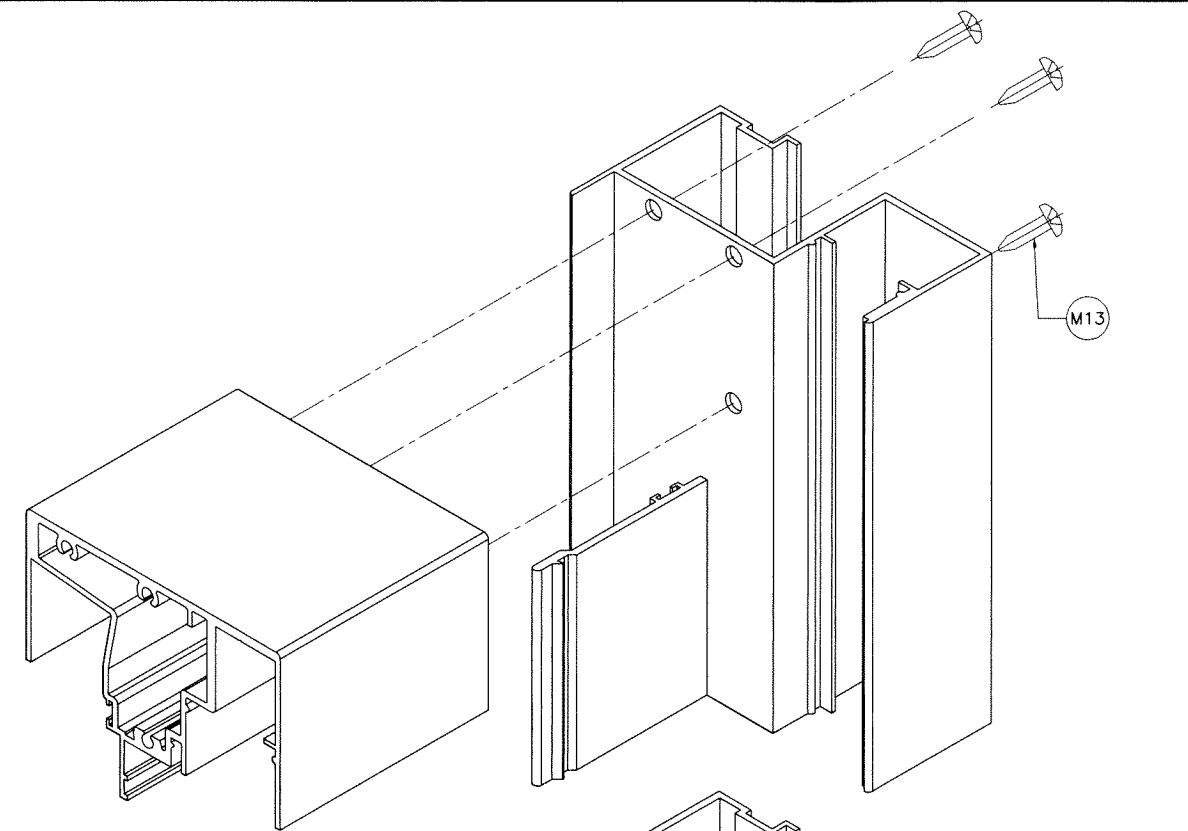
FRAME TOP CORNER
