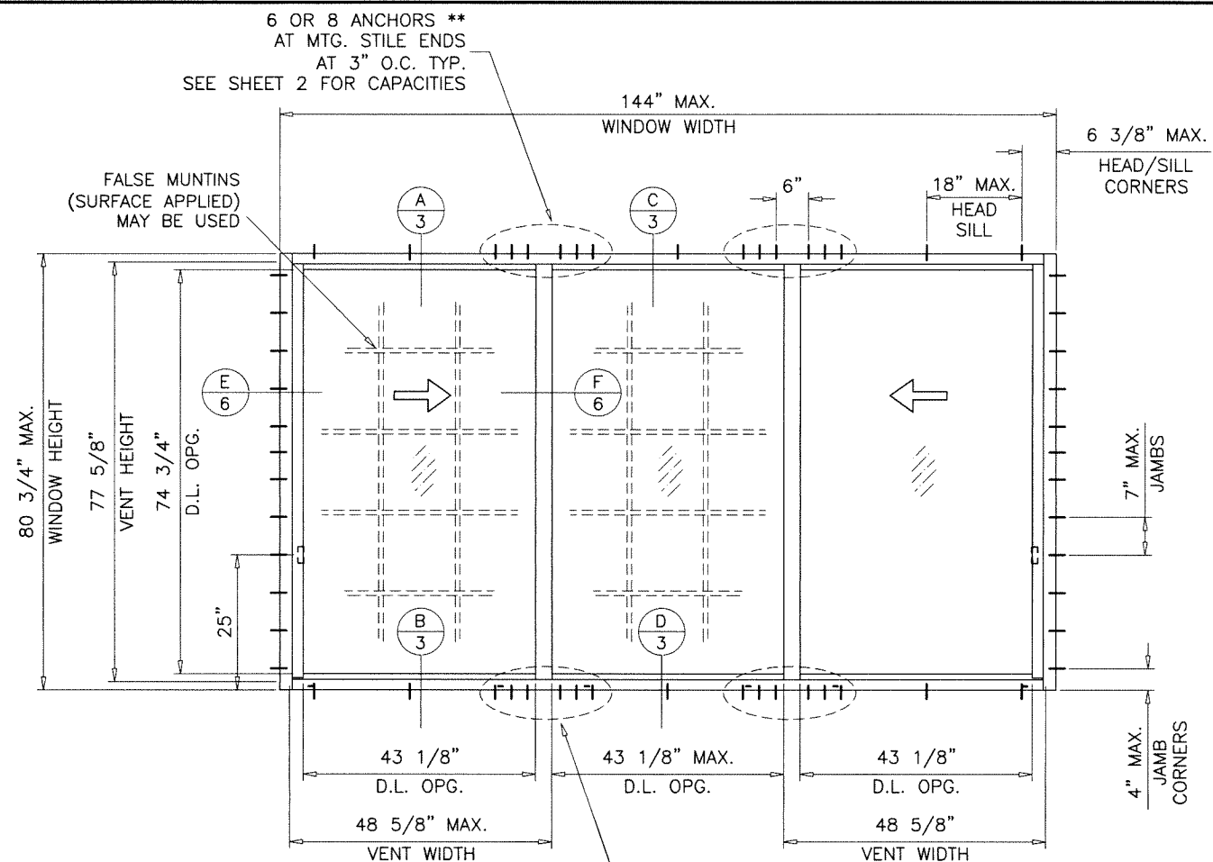
TYPICAL ELEVATIONS EQUAL LITES
